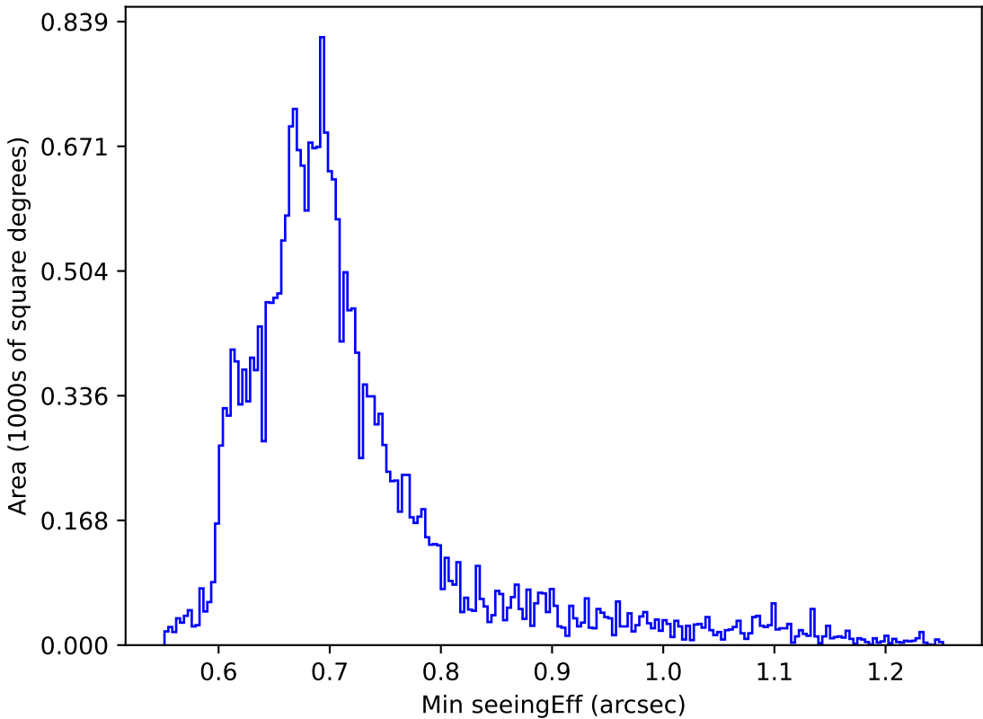
too_elab_r16_d3_ugrizy_v3.4_10yrs Yr 1 r band: Min seeingEff
