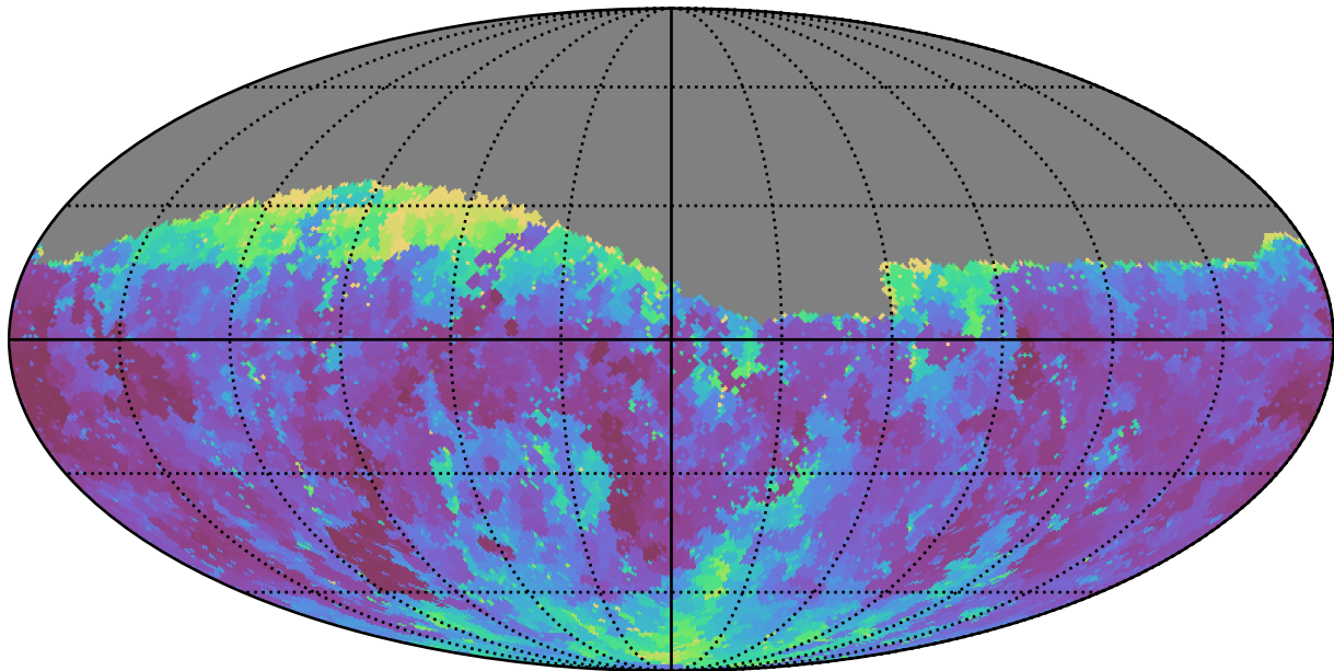
too_elab_r16_d3_ugrizy_v3.4_10yrs Yr 1 g band: Min seeingEff
