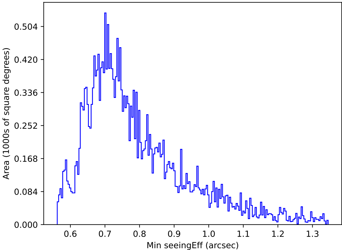
too_elab_r16_d3_ugrizy_v3.4_10yrs Yr 1 g band: Min seeingEff
