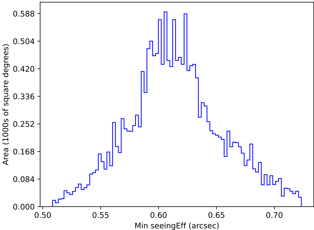
too_elab_r16_d3_ugrizy_v3.4_10yrs WFD z band: Min seeingEff
