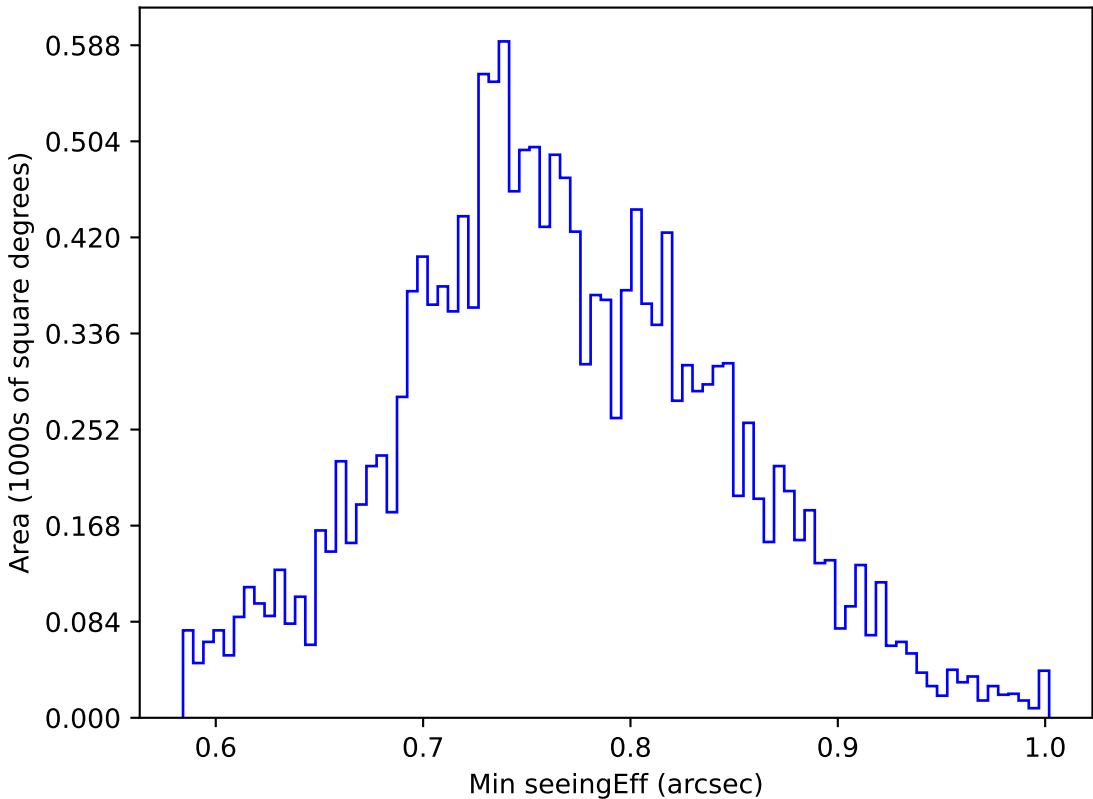
too_elab_r16_d3_ugrizy_v3.4_10yrs WFD u band: Min seeingEff
