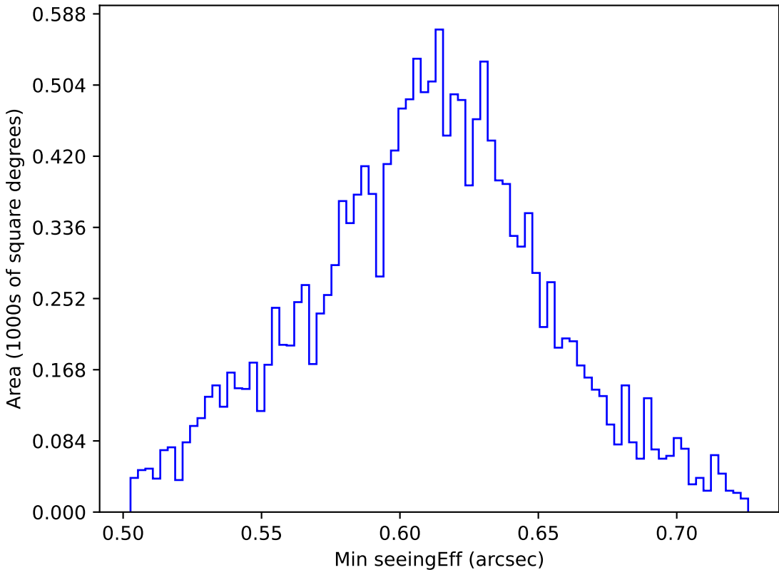
too_elab_r16_d3_ugrizy_v3.4_10yrs WFD r band: Min seeingEff
