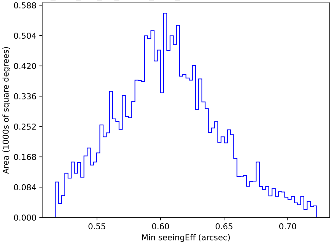
too_elab_r16_d3_ugrizy_v3.4_10yrs WFD i band: Min seeingEff
