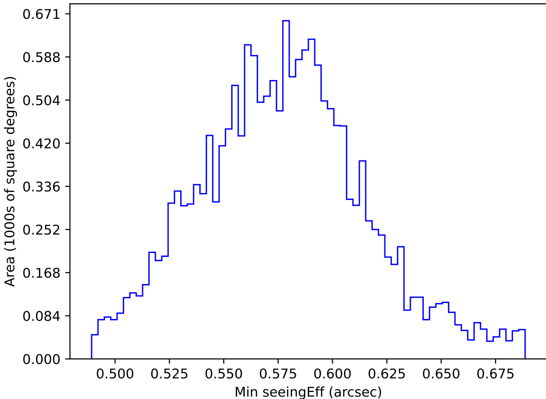
too_elab_r16_d3_ugrizy_v3.4_10yrs WFD all bands: Min seeingEff
