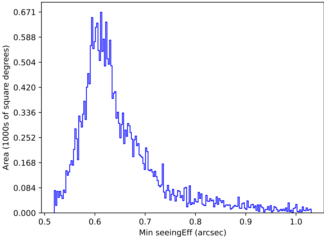
too_elab_r16_d3_ugrizy_v3.4_10yrs All sky z band: Min seeingEff
