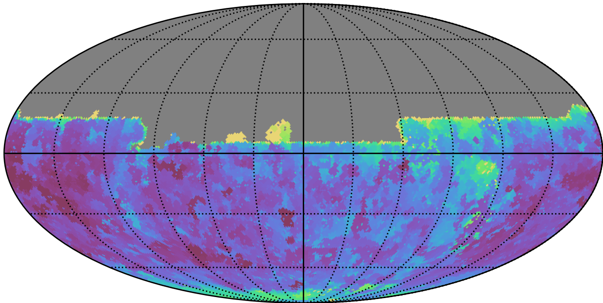
too_elab_r16_d3_ugrizy_v3.4_10yrs All sky u band: Min seeingEff
