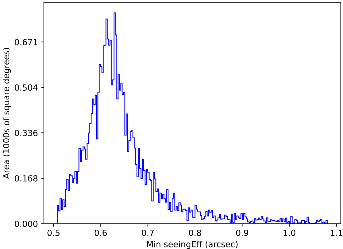
too_elab_r16_d3_ugrizy_v3.4_10yrs All sky r band: Min seeingEff
