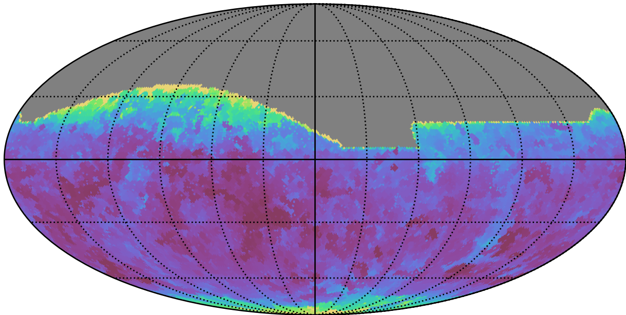
too_elab_r16_d3_ugrizy_v3.4_10yrs All sky i band: Min seeingEff
