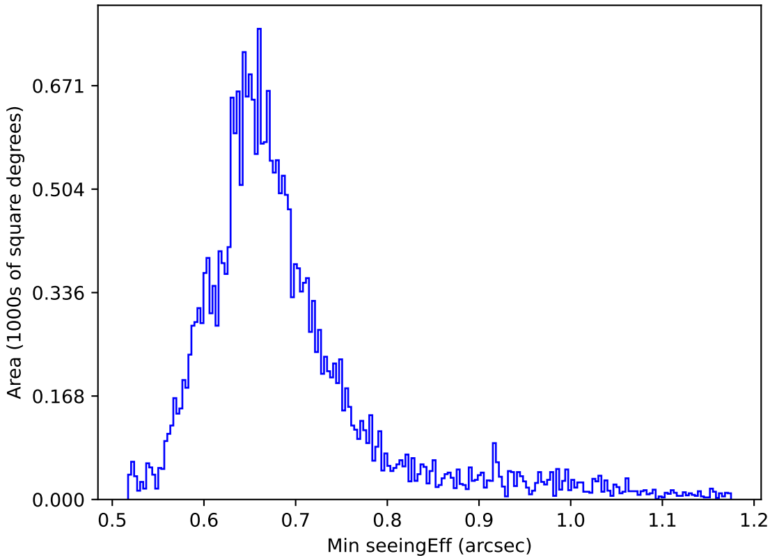
too_elab_r16_d3_ugrizy_v3.4_10yrs All sky g band: Min seeingEff
