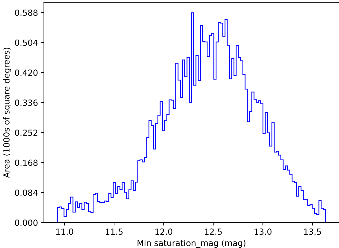
too_elab_r16_d3_ugrizy_v3.4_10yrs All sky i band: Min saturation_mag
