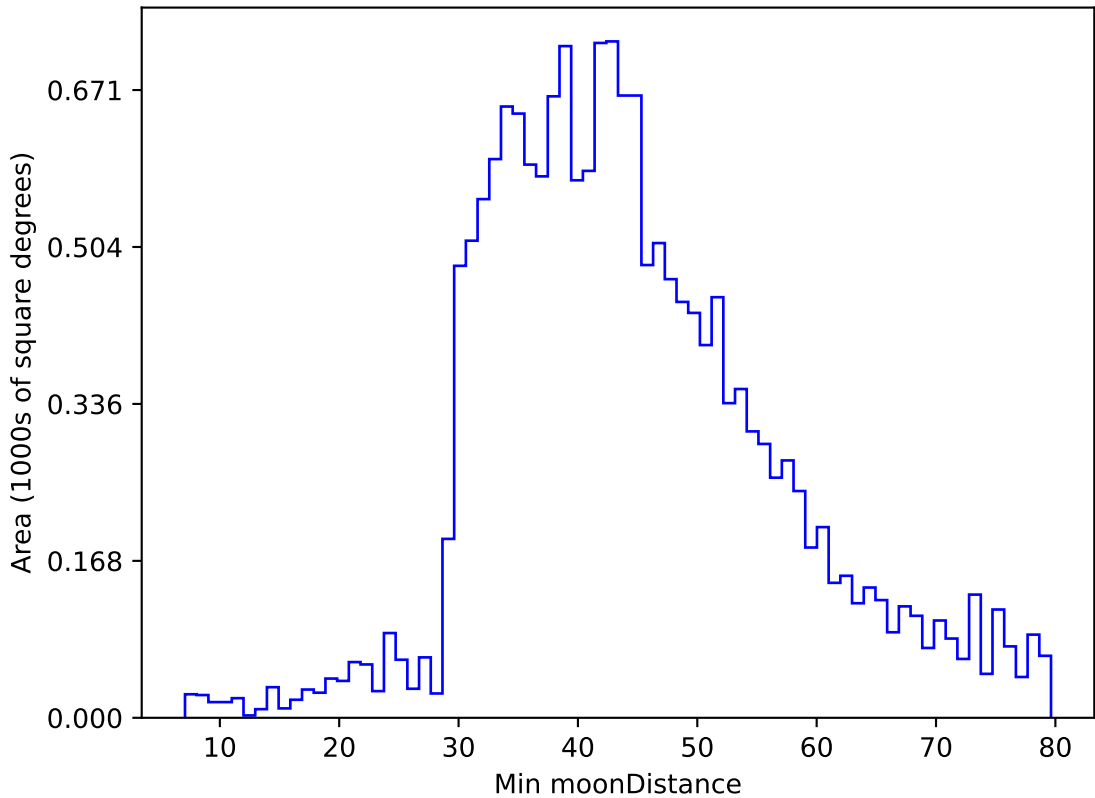
too_elab_r16_d3_ugrizy_v3.4_10yrs WFD g band: Min moonDistance
