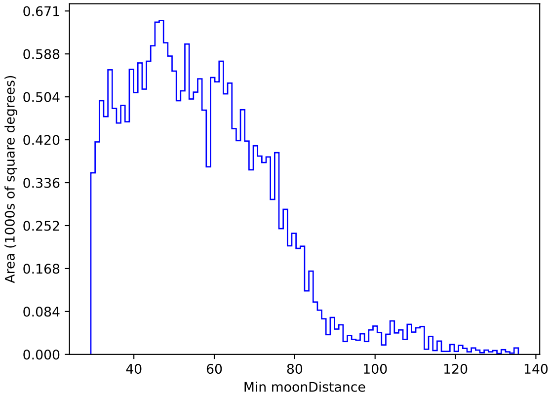
too_elab_r16_d3_ugrizy_v3.4_10yrs All sky u band: Min moonDistance
