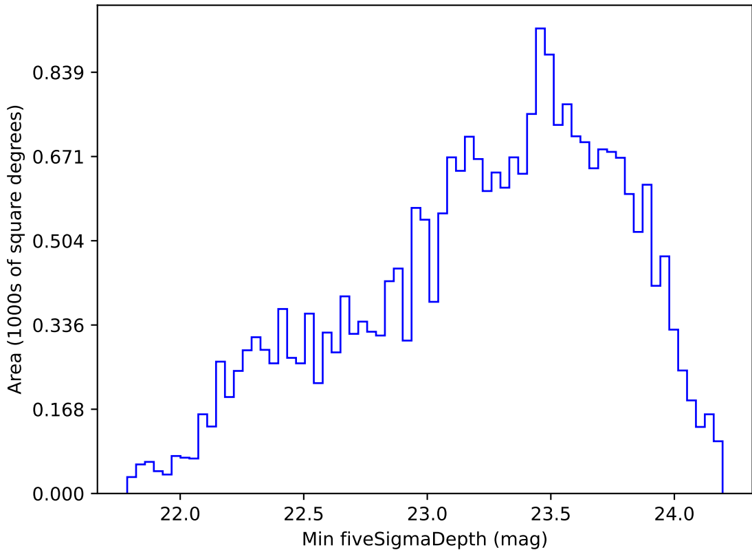
too_elab_r16_d3_ugrizy_v3.4_10yrs Yr 1 r band: Min fiveSigmaDepth
