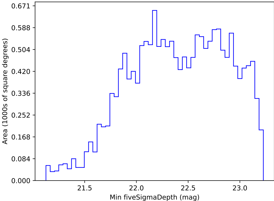
too_elab_r16_d3_ugrizy_v3.4_10yrs WFD r band: Min fiveSigmaDepth
