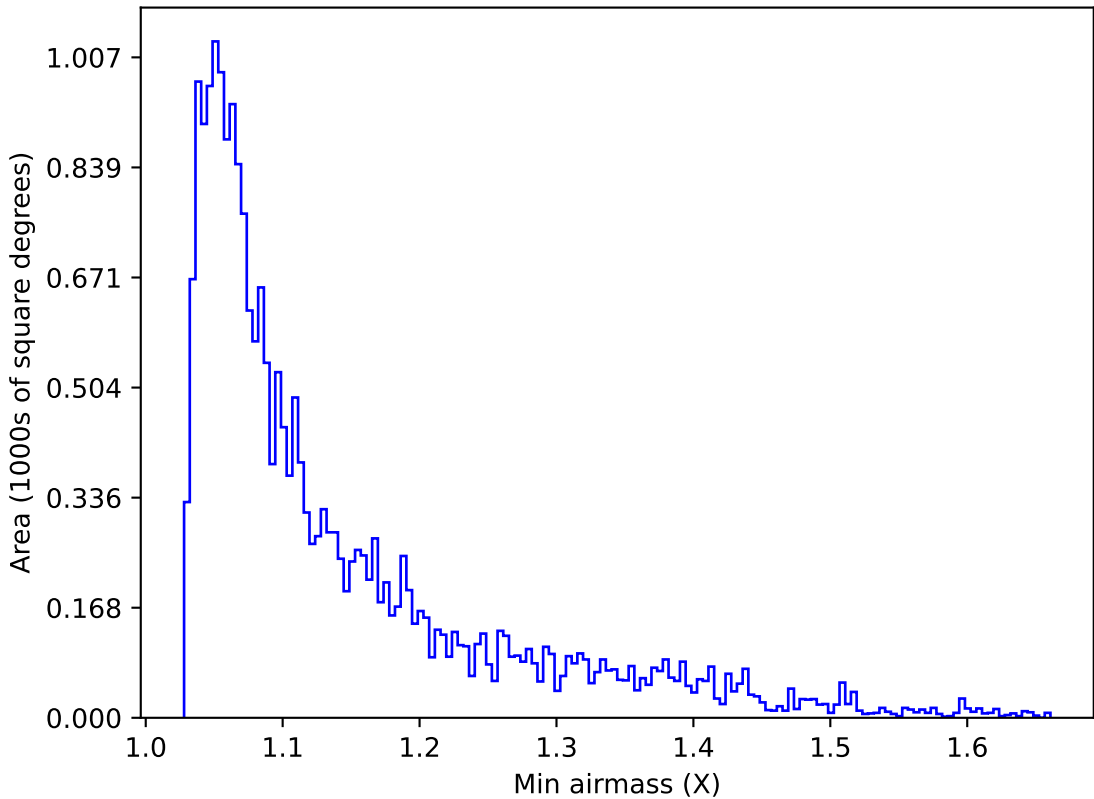
too_elab_r16_d3_ugrizy_v3.4_10yrs Yr 1 u band: Min airmass
