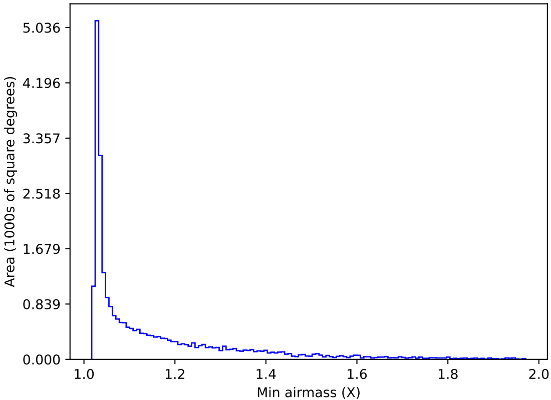
too_elab_r16_d3_ugrizy_v3.4_10yrs Yr 1 all bands: Min airmass
