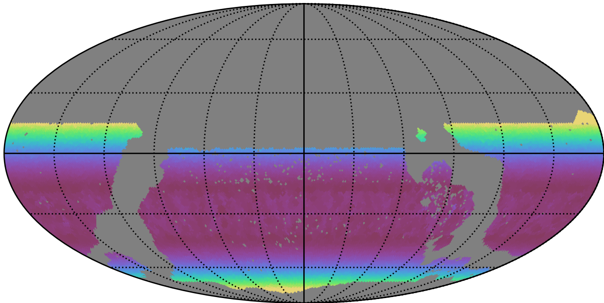
too_elab_r16_d3_ugrizy_v3.4_10yrs WFD u band: Min airmass
