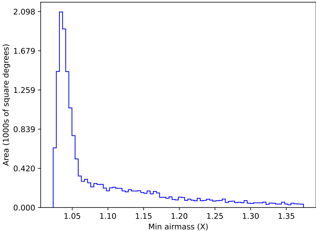
too_elab_r16_d3_ugrizy_v3.4_10yrs WFD u band: Min airmass
