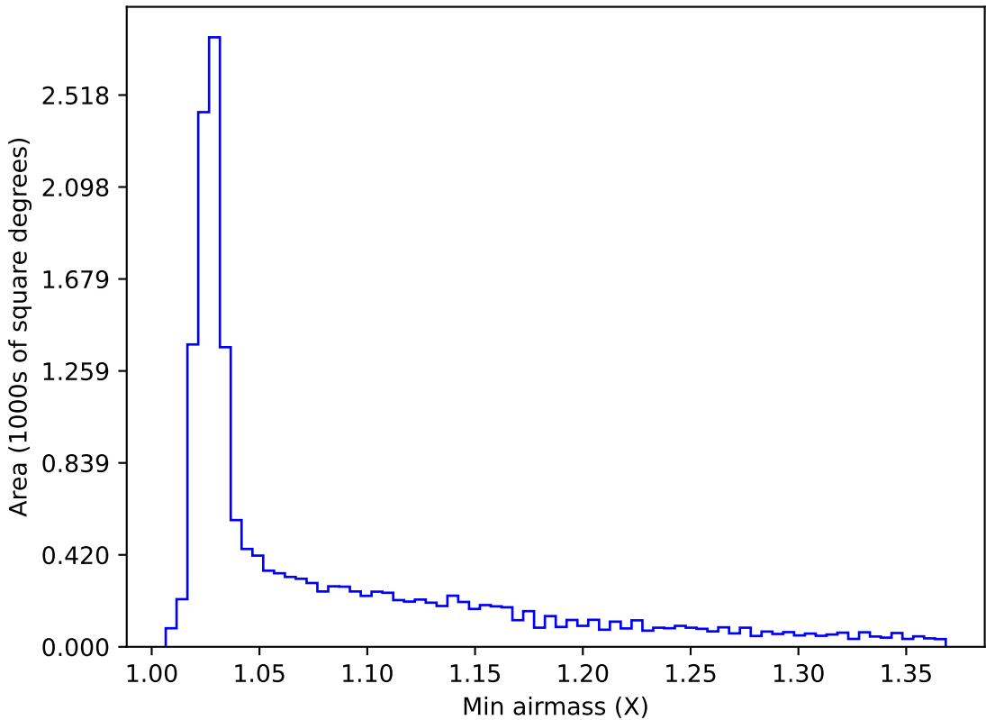
too_elab_r16_d3_ugrizy_v3.4_10yrs WFD r band: Min airmass
