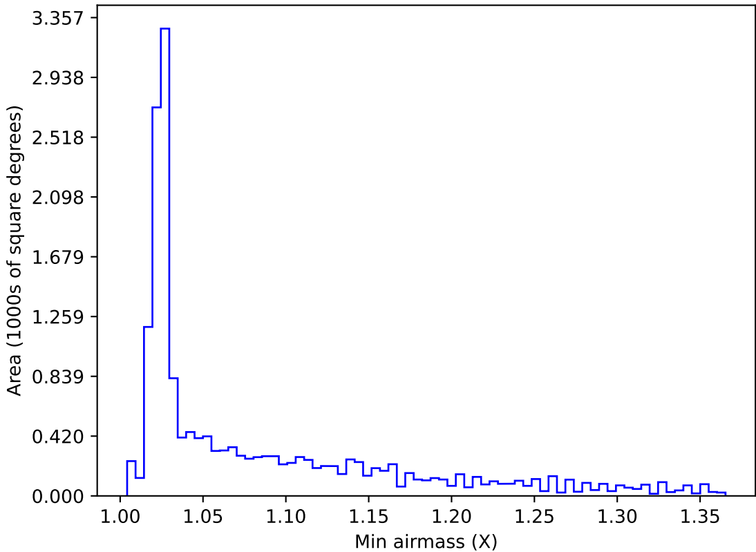
too_elab_r16_d3_ugrizy_v3.4_10yrs WFD all bands: Min airmass
