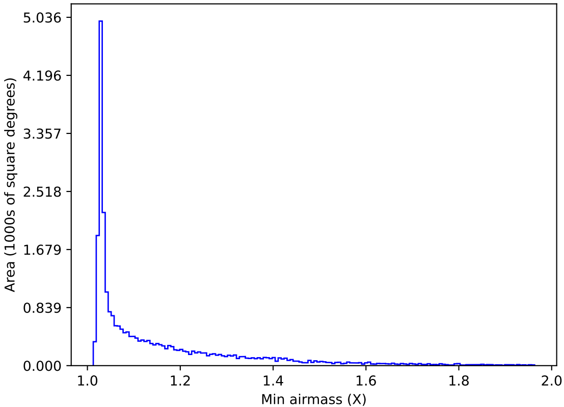
too_elab_r16_d3_ugrizy_v3.4_10yrs All sky z band: Min airmass
