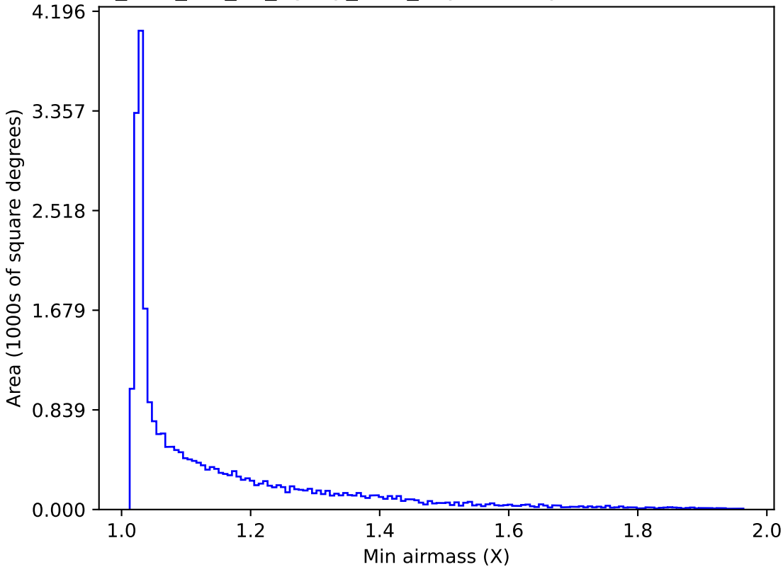
too_elab_r16_d3_ugrizy_v3.4_10yrs All sky r band: Min airmass
