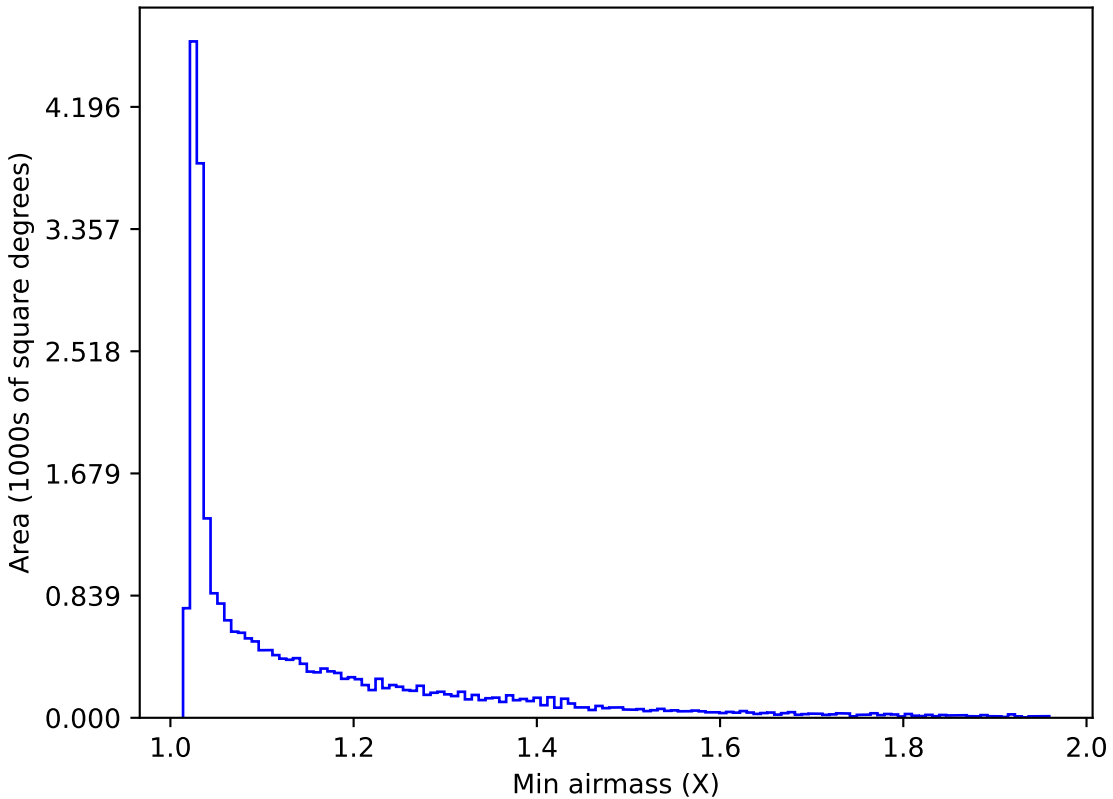
too_elab_r16_d3_ugrizy_v3.4_10yrs All sky i band: Min airmass
