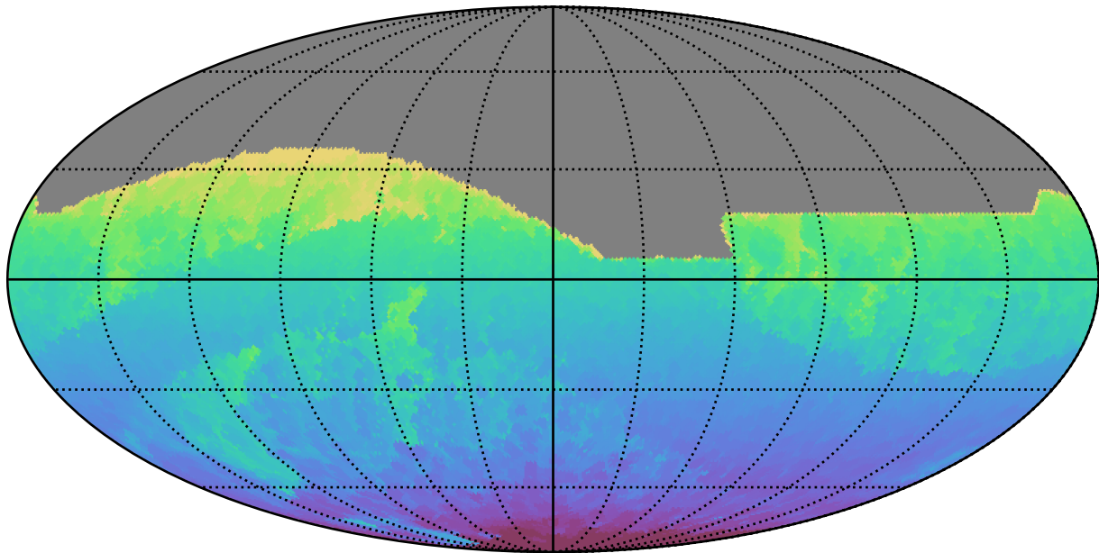
too_elab_r16_d3_ugrizy_v3.4_10yrs All sky all bands: Min HA
