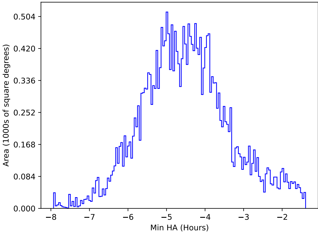
too_elab_r16_d3_ugrizy_v3.4_10yrs All sky all bands: Min HA
