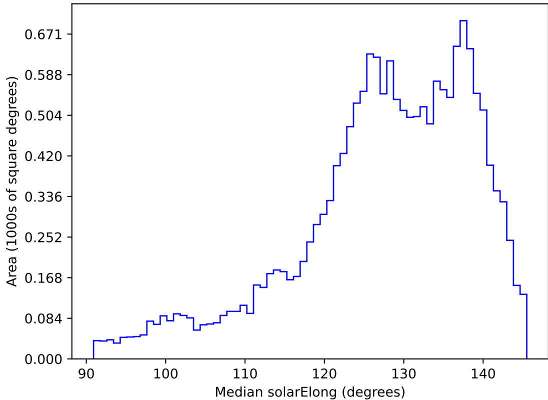
too_elab_r16_d3_ugrizy_v3.4_10yrs WFD z band: Median solarElong
