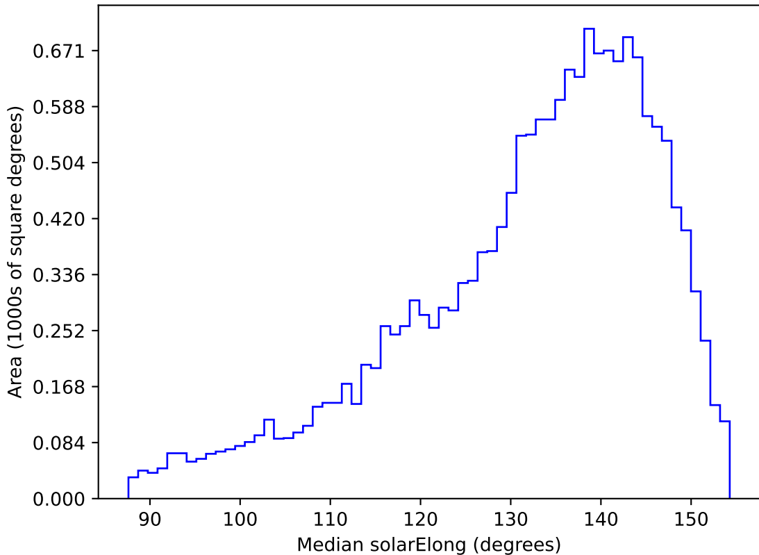
too_elab_r16_d3_ugrizy_v3.4_10yrs WFD u band: Median solarElong
