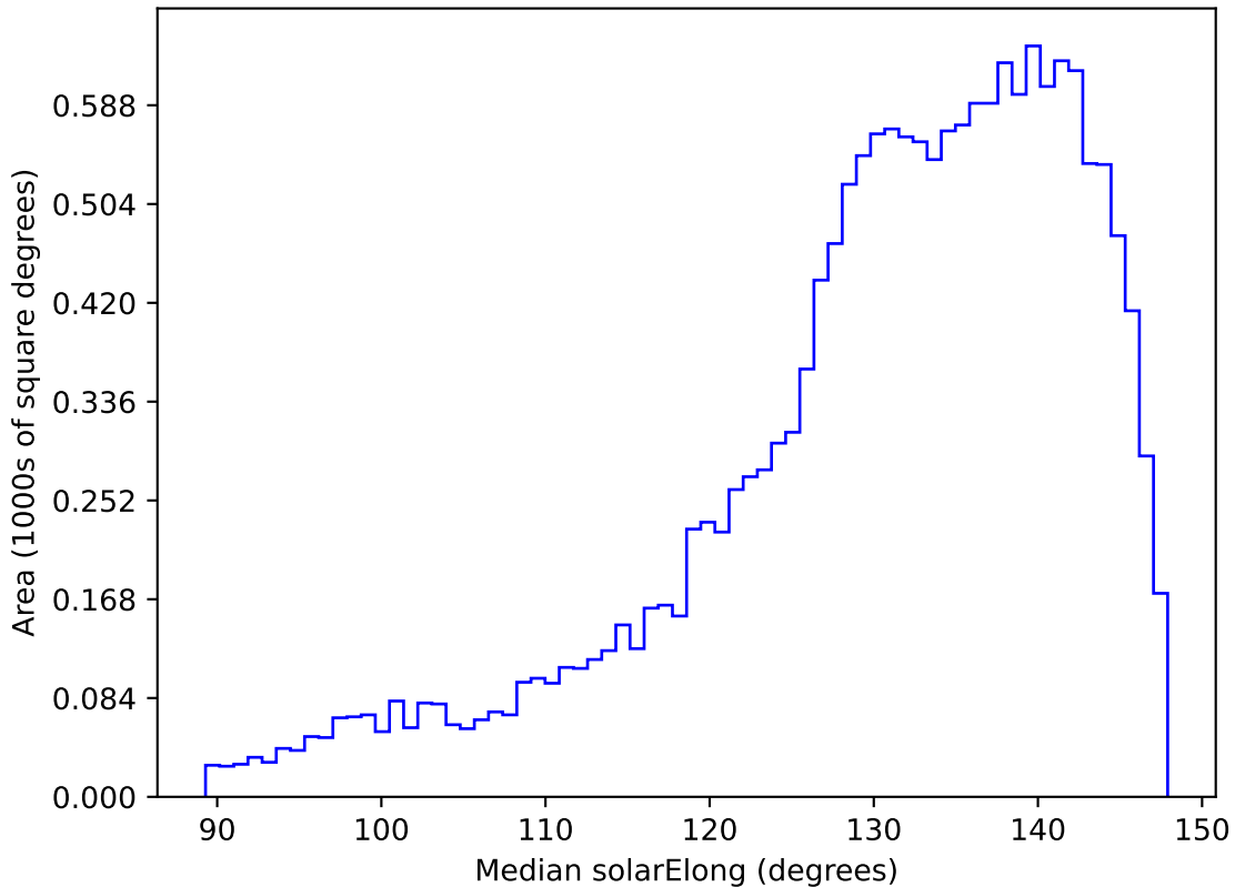
too_elab_r16_d3_ugrizy_v3.4_10yrs WFD r band: Median solarElong
