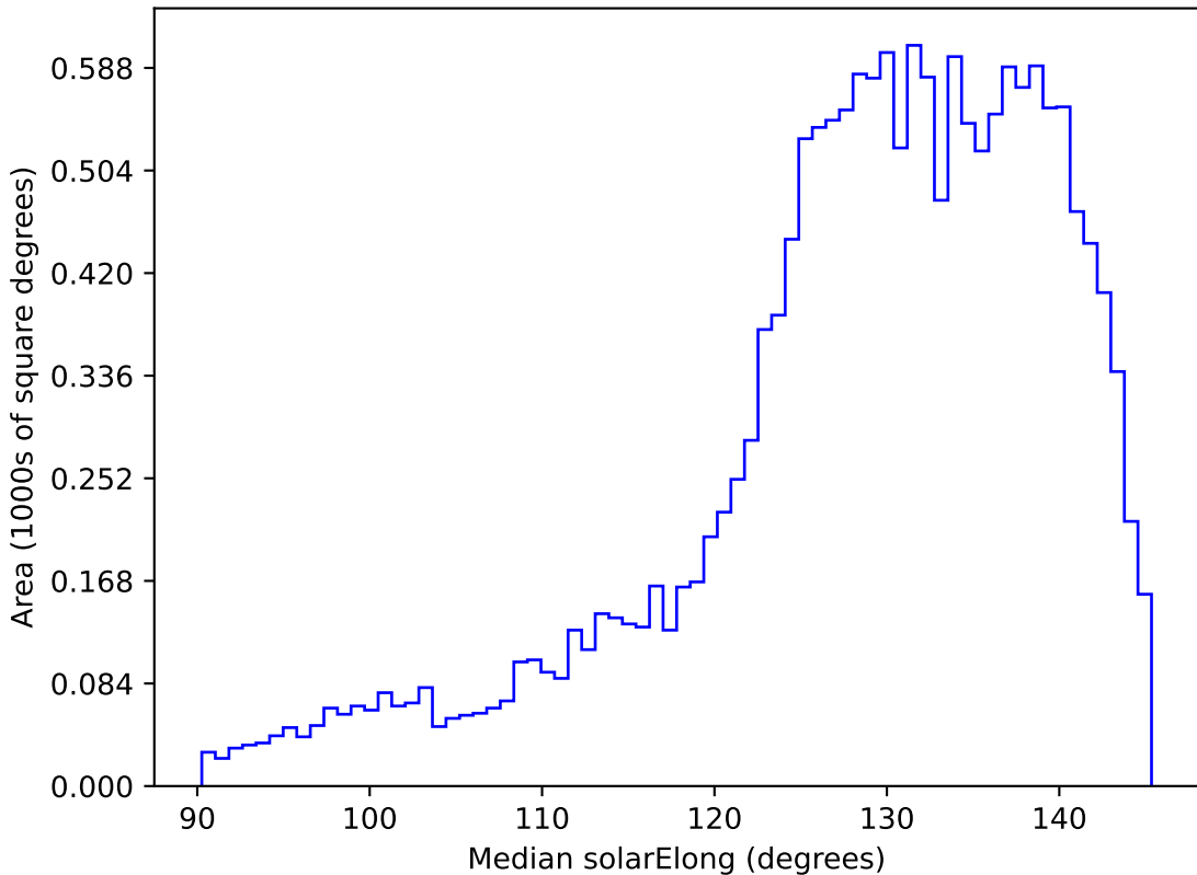
too_elab_r16_d3_ugrizy_v3.4_10yrs WFD i band: Median solarElong
