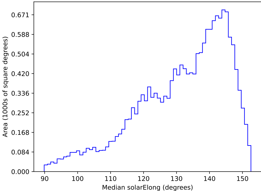
too_elab_r16_d3_ugrizy_v3.4_10yrs WFD g band: Median solarElong
