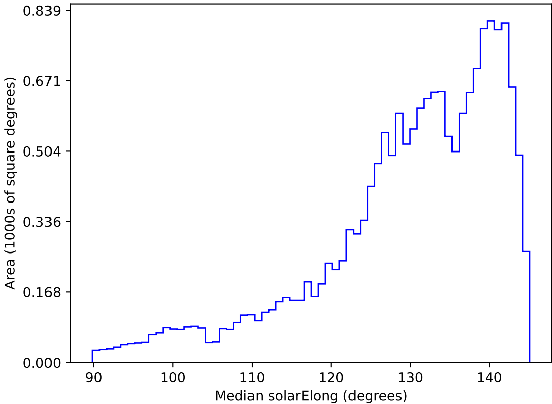
too_elab_r16_d3_ugrizy_v3.4_10yrs WFD all bands: Median solarElong
