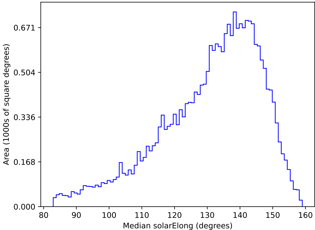
too_elab_r16_d3_ugrizy_v3.4_10yrs All sky u band: Median solarElong
