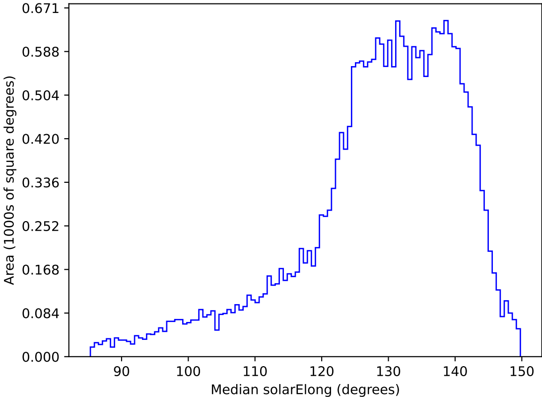
too_elab_r16_d3_ugrizy_v3.4_10yrs All sky i band: Median solarElong
