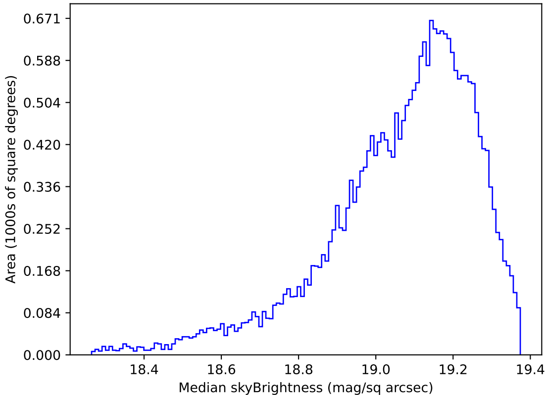
too_elab_r16_d3_ugrizy_v3.4_10yrs Yr 1 z band: Median skyBrightness
