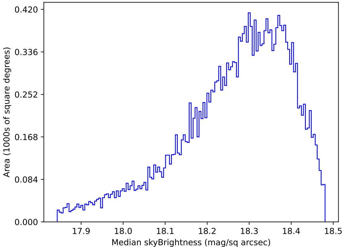
too_elab_r16_d3_ugrizy_v3.4_10yrs Yr 1 y band: Median skyBrightness
