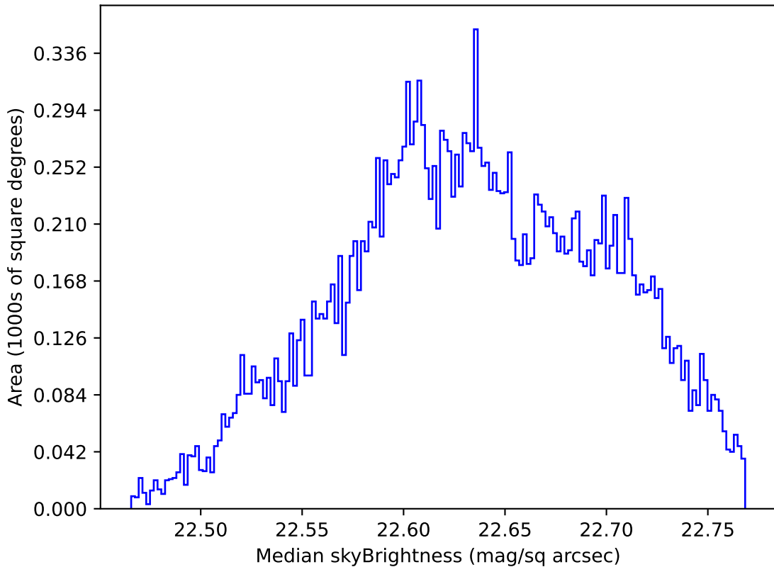
too_elab_r16_d3_ugrizy_v3.4_10yrs Yr 1 u band: Median skyBrightness
