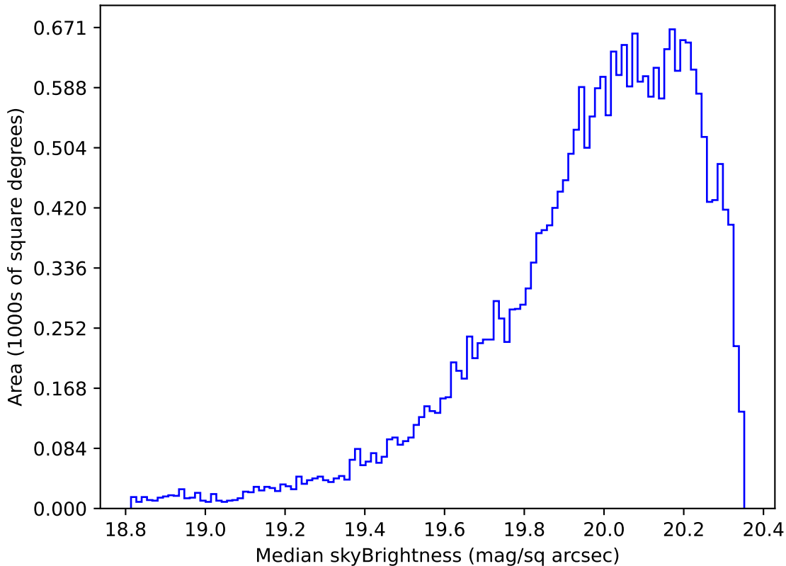
too_elab_r16_d3_ugrizy_v3.4_10yrs Yr 1 i band: Median skyBrightness
