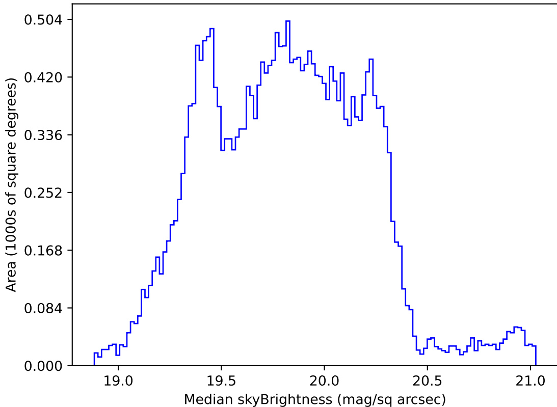
too_elab_r16_d3_ugrizy_v3.4_10yrs Yr 1 all bands: Median skyBrightness
