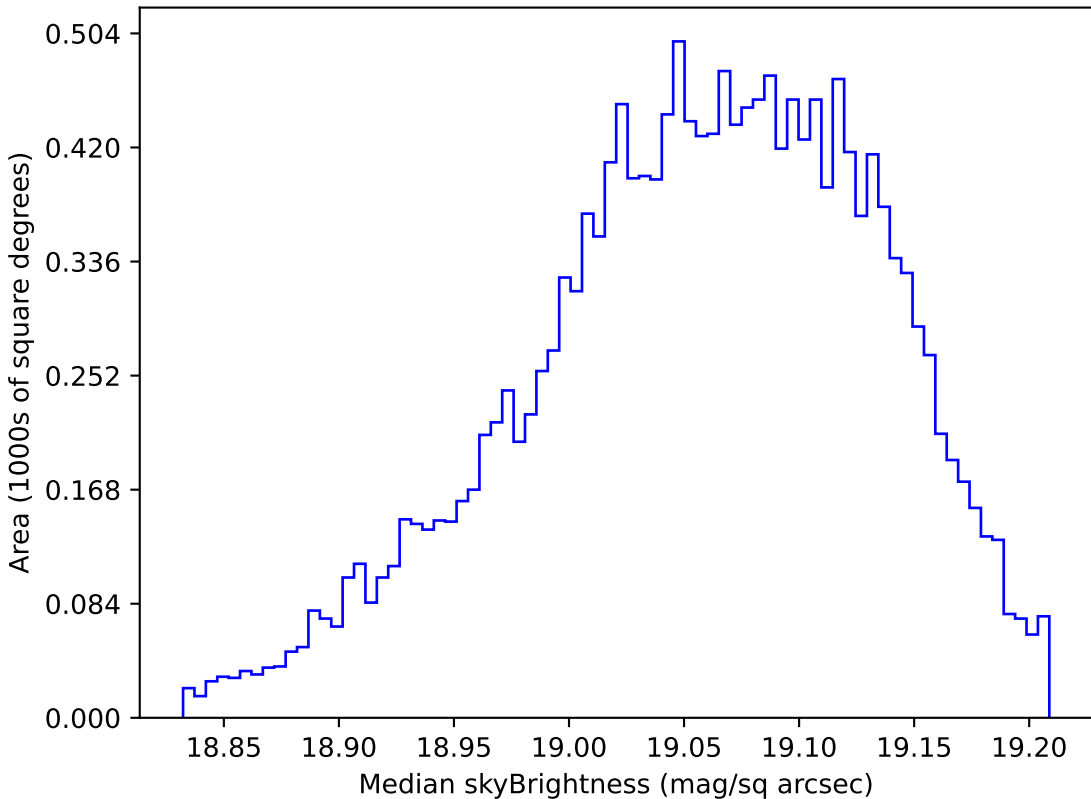
too_elab_r16_d3_ugrizy_v3.4_10yrs WFD z band: Median skyBrightness
