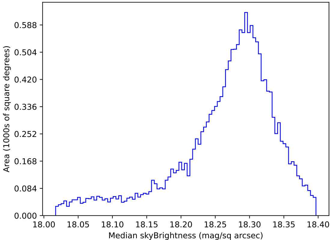
too_elab_r16_d3_ugrizy_v3.4_10yrs WFD y band: Median skyBrightness
