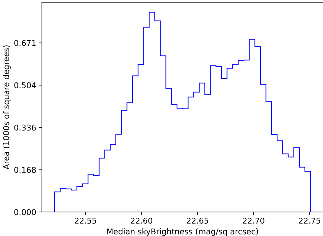
too_elab_r16_d3_ugrizy_v3.4_10yrs WFD u band: Median skyBrightness
