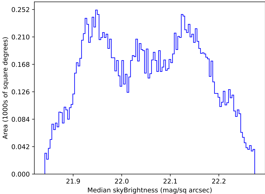
too_elab_r16_d3_ugrizy_v3.4_10yrs WFD g band: Median skyBrightness
