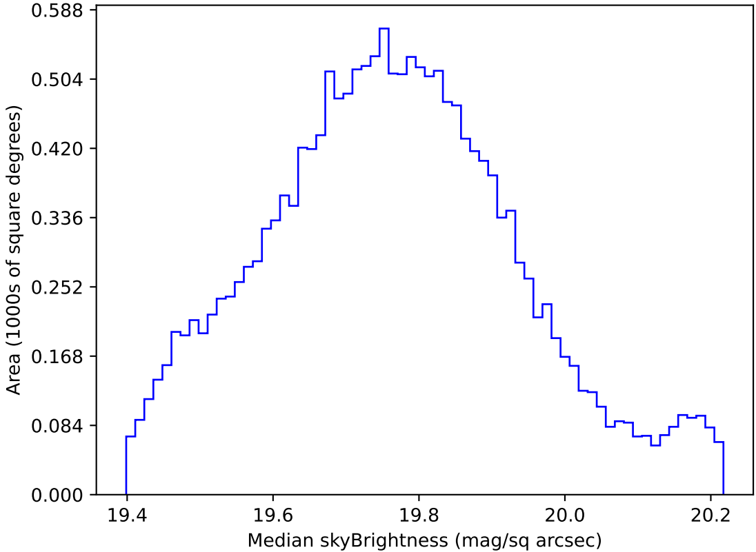
too_elab_r16_d3_ugrizy_v3.4_10yrs WFD all bands: Median skyBrightness
