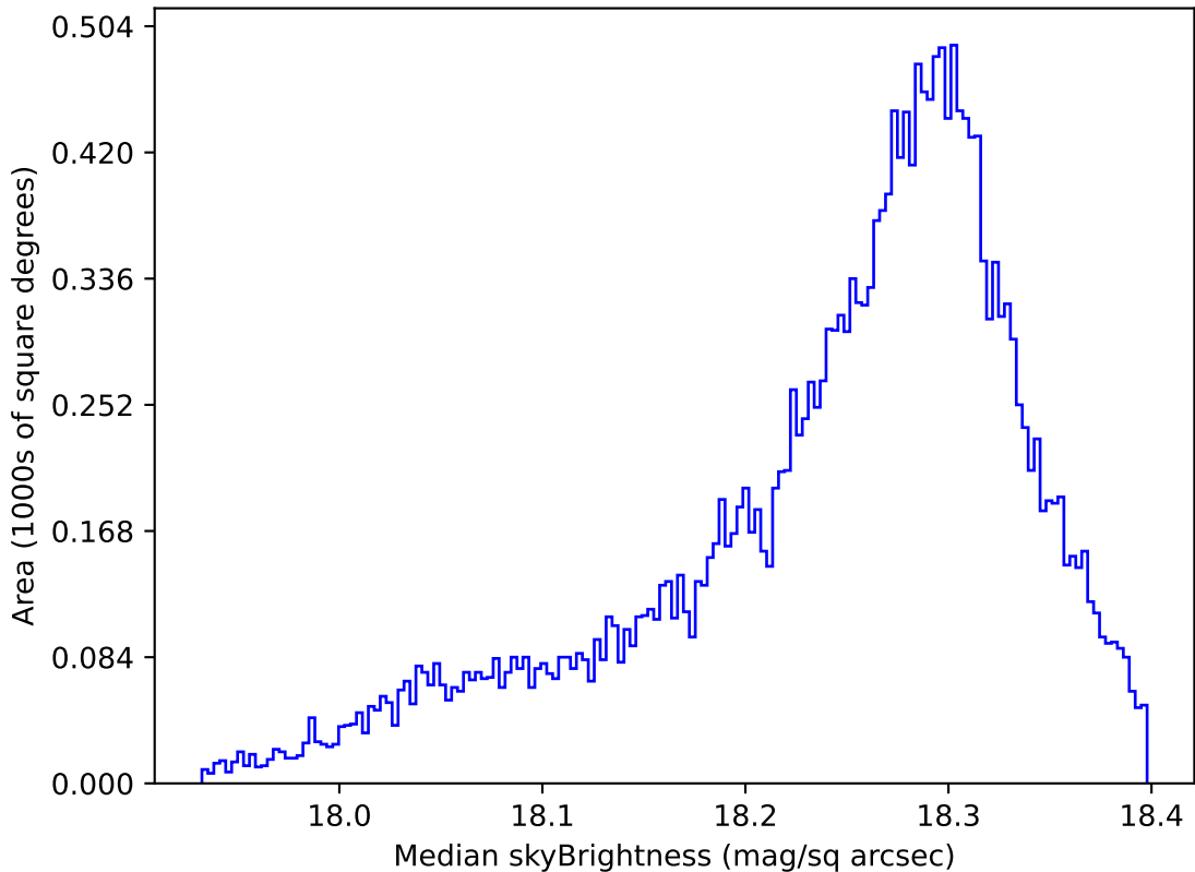
too_elab_r16_d3_ugrizy_v3.4_10yrs All sky y band: Median skyBrightness
