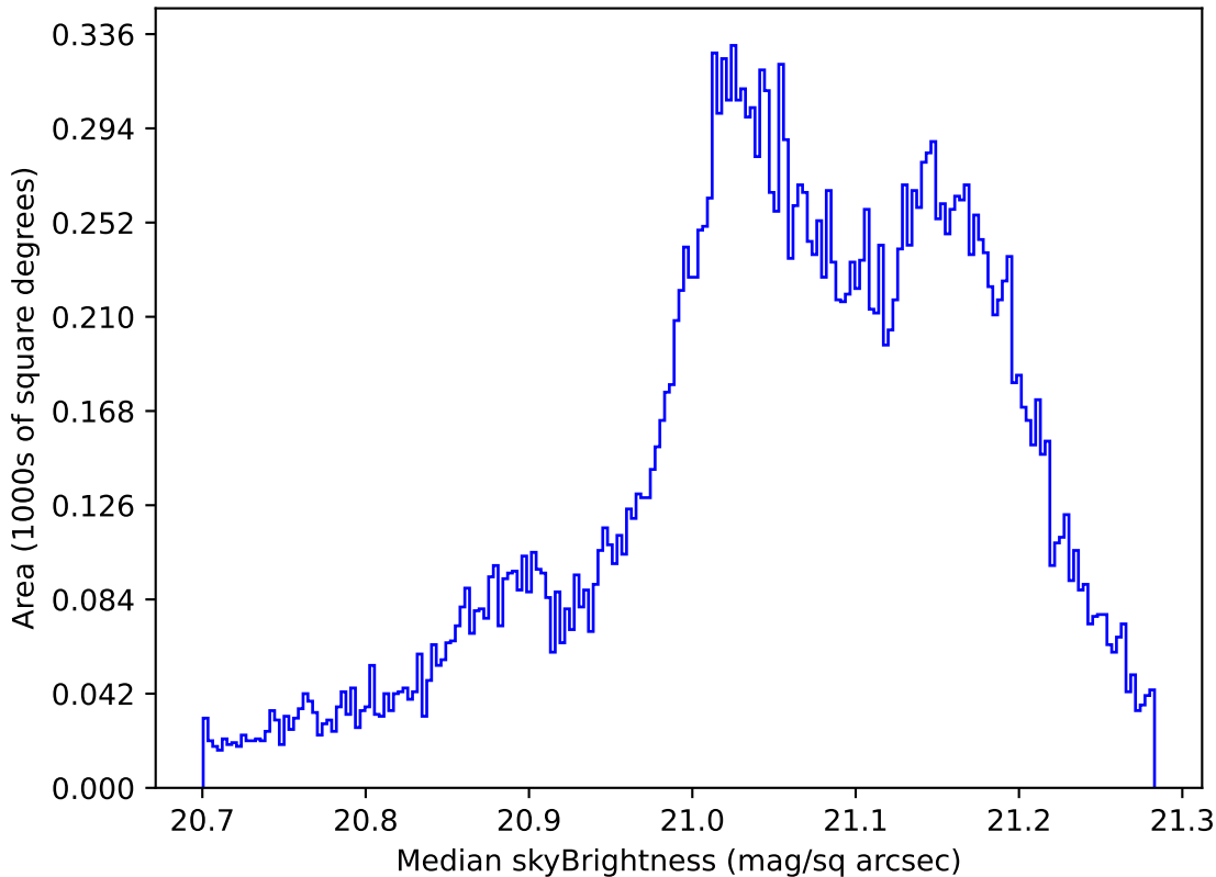
too_elab_r16_d3_ugrizy_v3.4_10yrs All sky r band: Median skyBrightness
