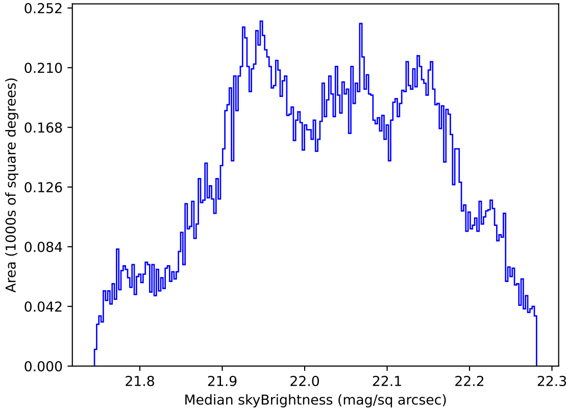
too_elab_r16_d3_ugrizy_v3.4_10yrs All sky g band: Median skyBrightness
